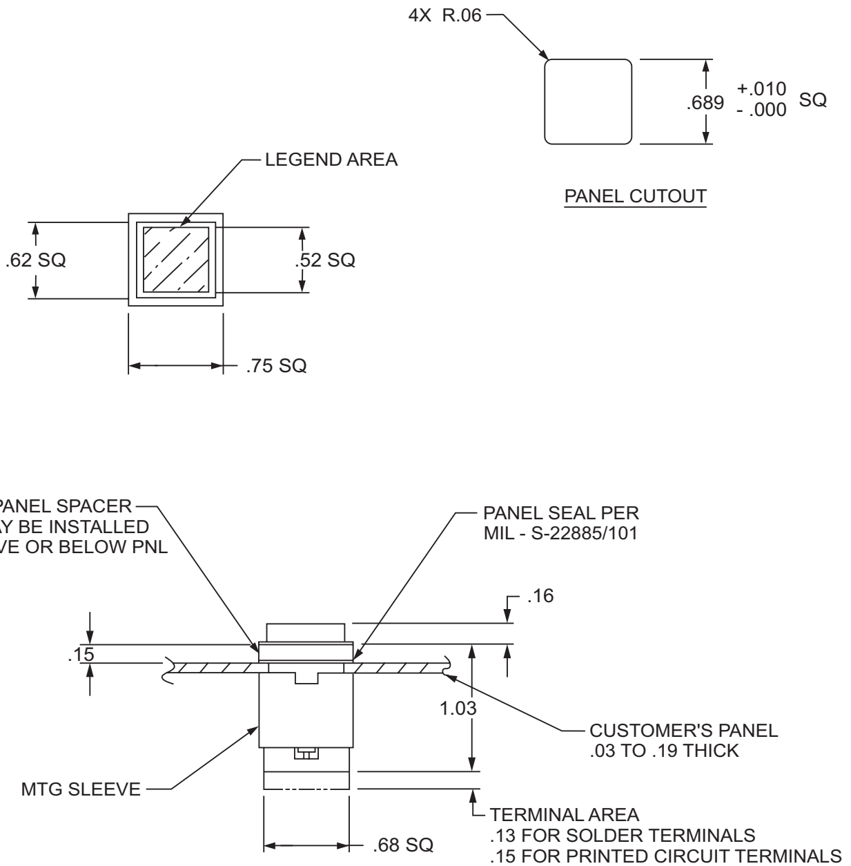
INTERNAL-SEAL SWITCH AND PUSHBUTTON ASSY (DRIP PROOF)
