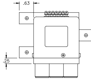
TN/TNH SWITCH
