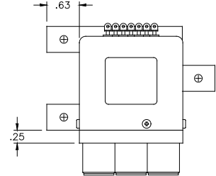
TT SWITCH
